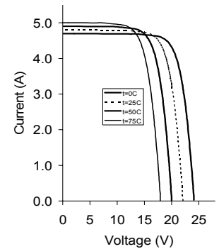
BP 380 I-V Curves
